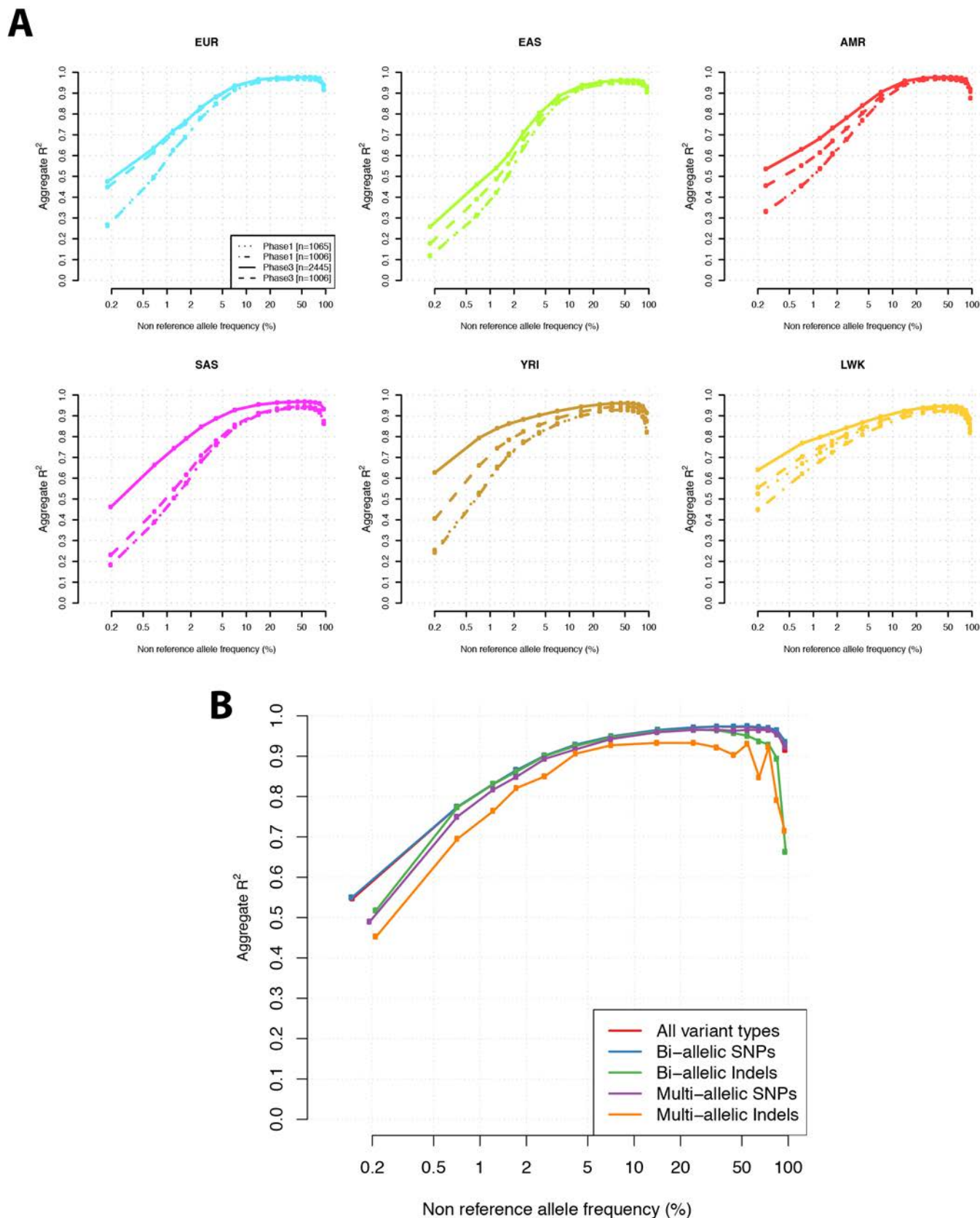
Extended Data Figure 9 | Performance of imputation. a , Performance of imputation in 6 populations using a subset of phase 3 as a reference panel ( n = 2,445 ), phase 1 ( n = 1,065 ), and the corresponding data within
